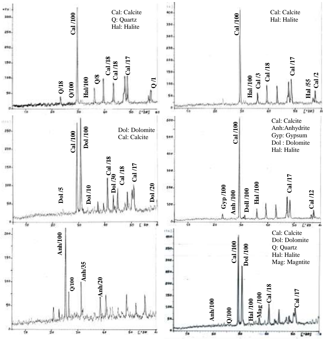
Fig. (20a- g) show the XRD patterns of investigated limestone samples.
