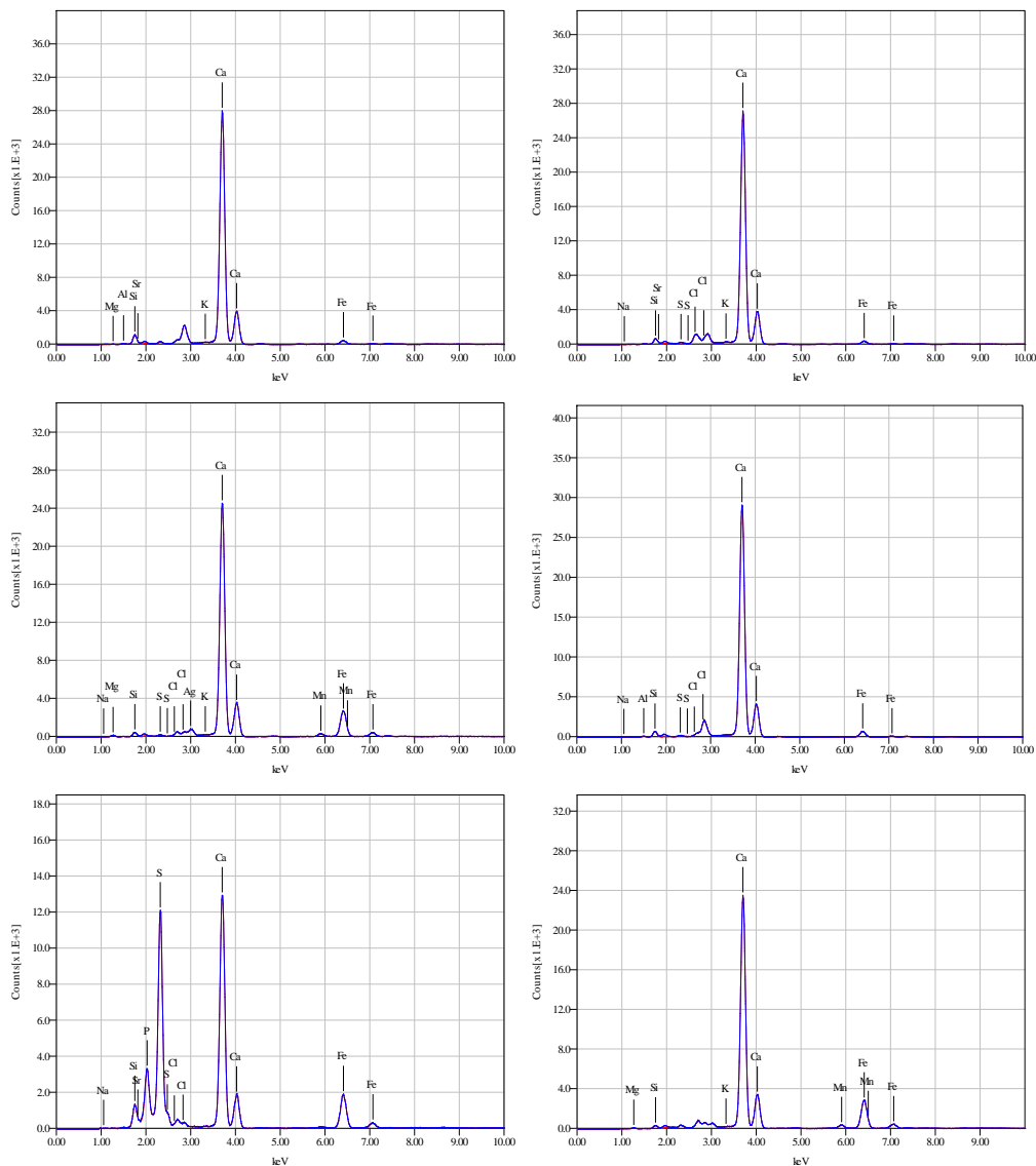
Figure 19 shows EDX patterns of the engraved limestone samples from Abu Musa excavation.
