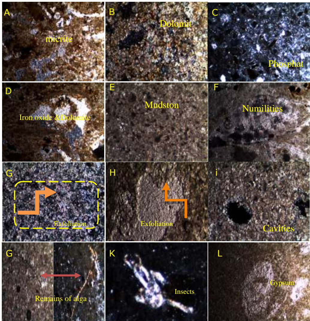
Figure(17) The examination of the limestone samples under polarized microscope shows a fine grained calcite (micrite), b Dolomite and iron oxides, c phosphate, d iron oxide and dolomite e mudstone f Numilities, g,h micro-exfoliation of calcite grains, i cavities and variety of cracking in calcite grains g remains of alga, k remains of insects, l Gypsum crystals.
